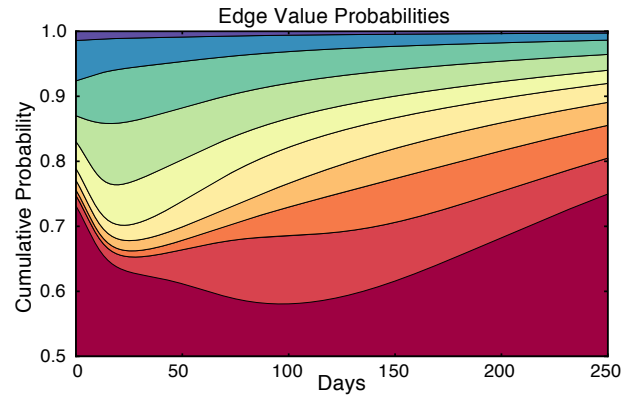
Figure 4: Edge value probabilities over time, with all other features kept equal. Values increase from 0 at bottom to 1 at top. Note that y axis starts at 0.5.
